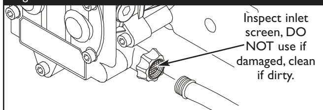
Figure 8 — Connect Garden Hose to Water Inlet
